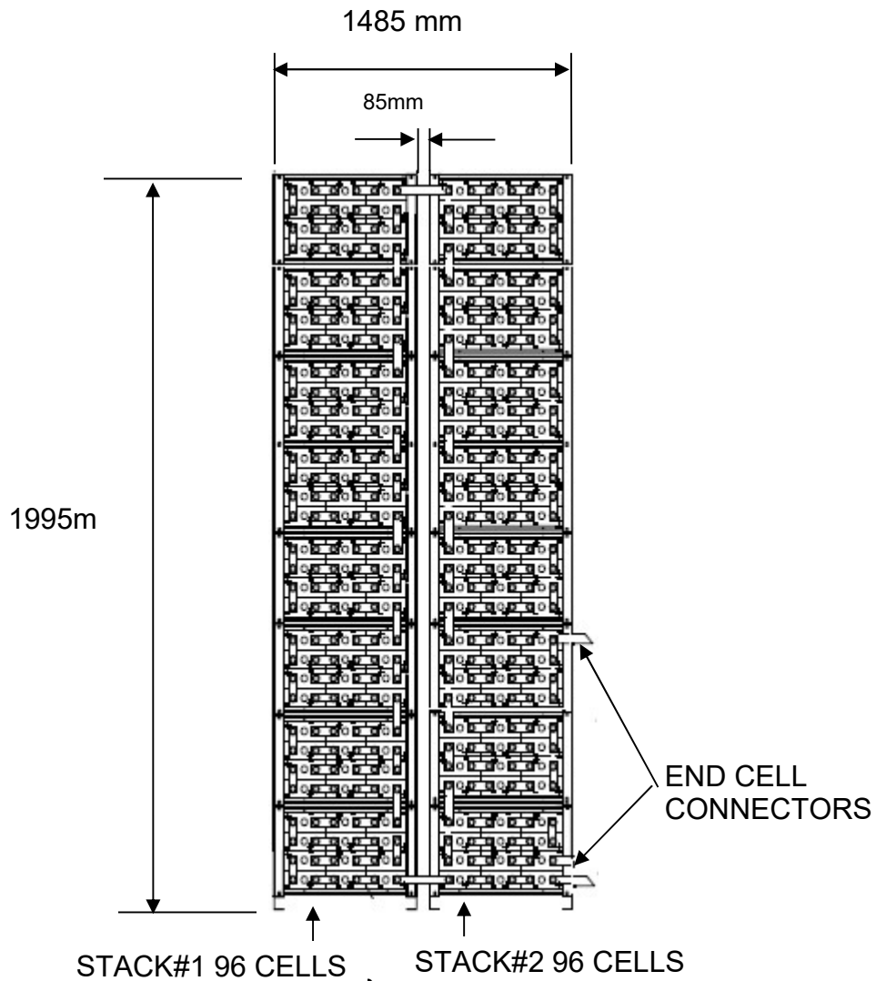
Reference diagram of Connection front view
